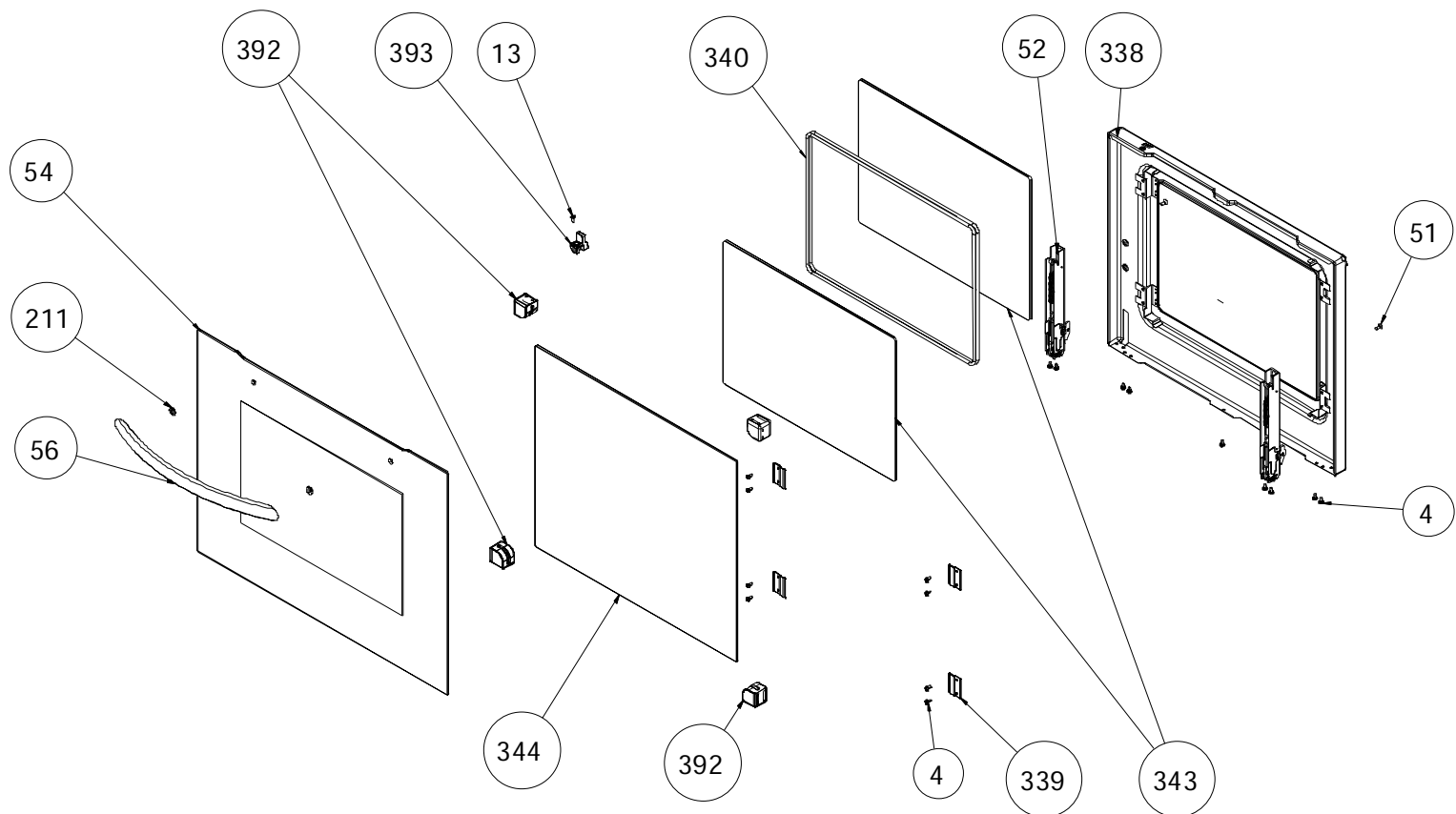
OVEN DOOR ASSEMBLY (OUTER & INNER) (POSITION NO 378)
