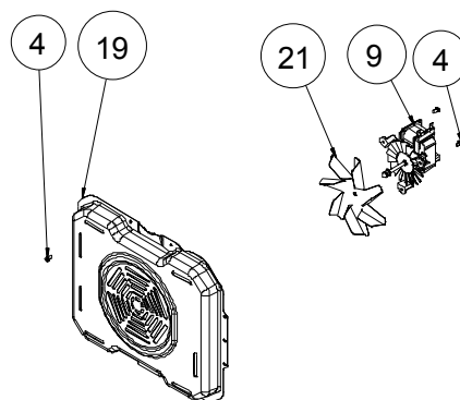
(FAN COVER/FAN IMPELLER ( 6 WINGS )/FAN MOTOR) (OPTIONAL)
